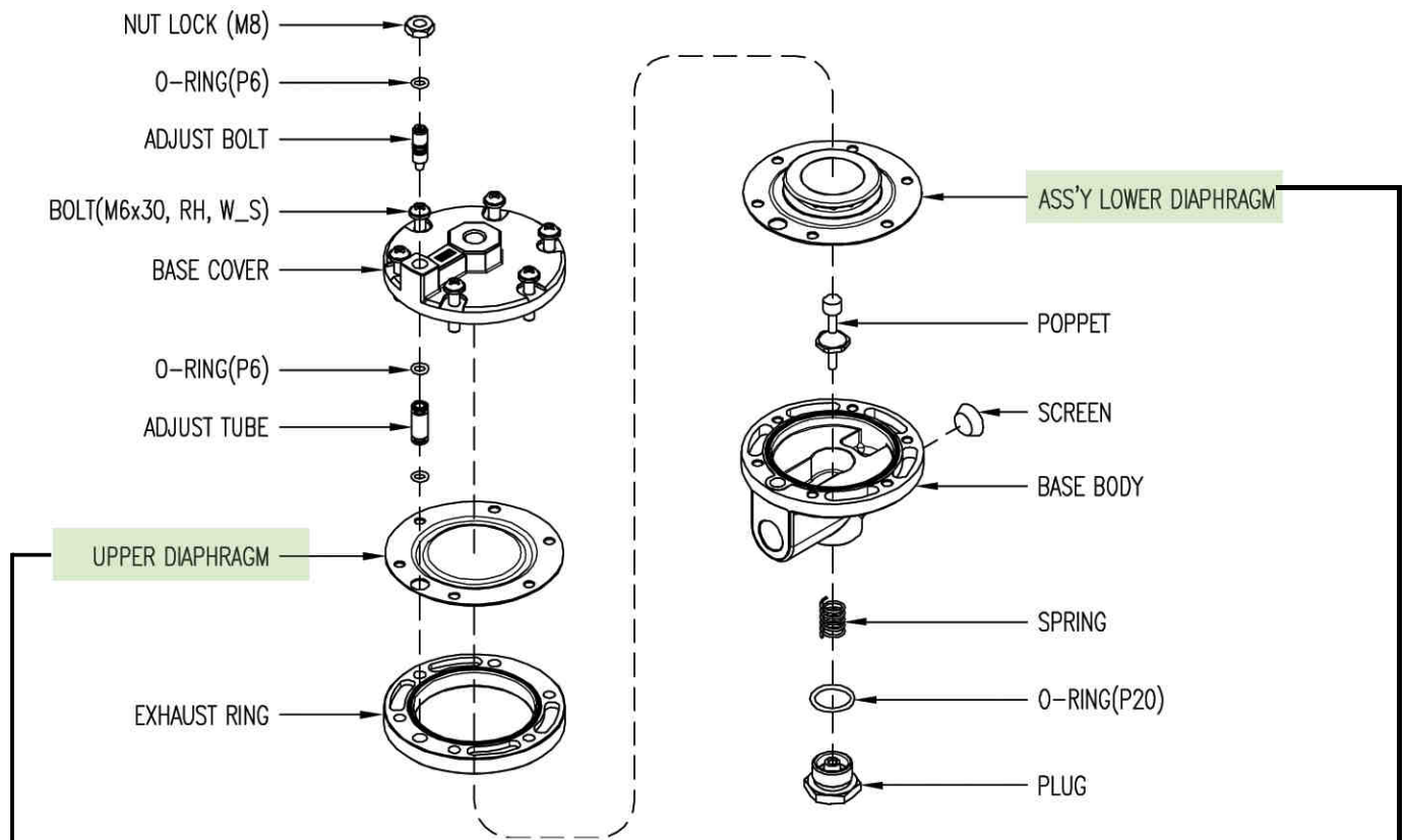
Fig. 2-4: YT-320 / 325 Parts and Assembly
