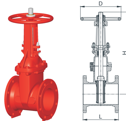
FIG. F0111-300, Size 2" to 12"
