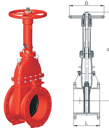
FIG. F1111-250, Size 14" to 18" FIG. F1111-200, Size 20" to 24"
